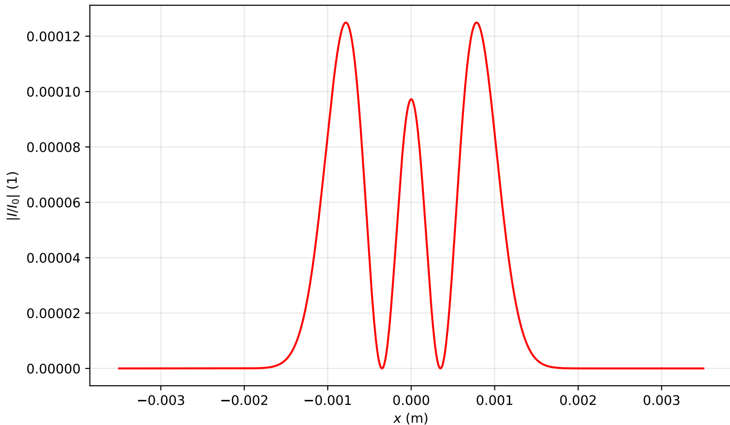
Intensity profile I(x, y = 0, z = 0.080)/I_0 , P_{in}=7.0P_{cr} , artificial time
